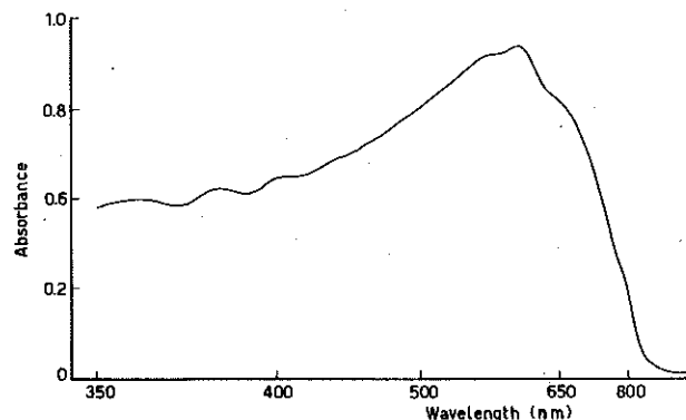
FIG. 1. Absorption spectrum (at room temperature) of soluble polyacetylene.
