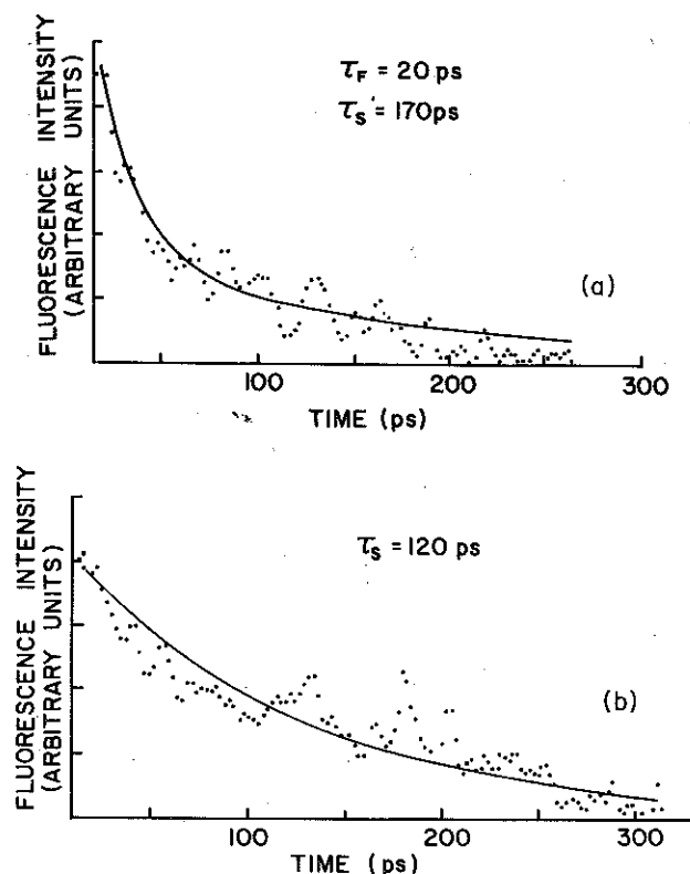
FIG. 3. Time-resolved emission spectrum of soluble polyacetylene, excitation 530 nm. (a) Emission for wavelengths > 540 \text{ nm} . (b) Emission for wavelengths > 580 \text{ nm} .
