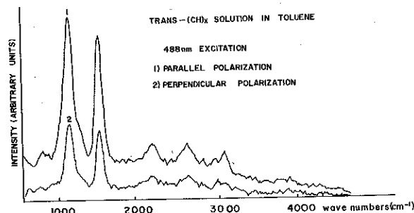
FIG. 2. Emission spectrum of soluble polyacetylene, excitation 488 nm. (1) Analyzer parallel to the polarization of the laser beam. (2) Analyzer perpendicular to the polarization of the laser beam.
