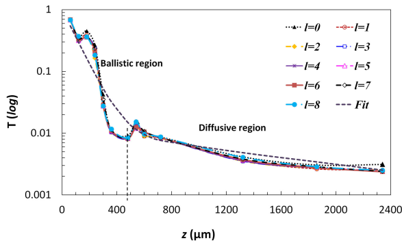
Figure 2 Transmittance ( T ) as a function of tissue thickness ( z ) at different topological charge l . Dashed curve is the theoretical fitting by equation T = e^{-\mu z} + Ce^{-\kappa z} , where \mu = 0.010403 \mu\text{m}^{-1} , C = 0.0112 , and \kappa = 6.3693 \times 10^{-4} \mu\text{m}^{-1} .
