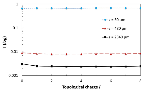
Figure 3 Transmission as a function of topological charge l of LG beams with tissue thickness z = 60 \mu\text{m} , 480 \mu\text{m} , and 2340 \mu\text{m} , respectively.
