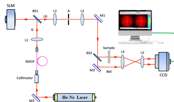
Figure 1 Experimental setup. SMOF, single mode optical fiber; L, lenses; G, Gaussian beam; BS, beam splitter; SLM, spatial light modulator; LG, Laguerre-Gaussian beam; A, aperture; M, mirrors; CCD, charge coupled device camera.
