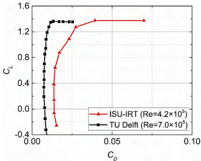
(b). Lift coefficients vs. drag coefficients
