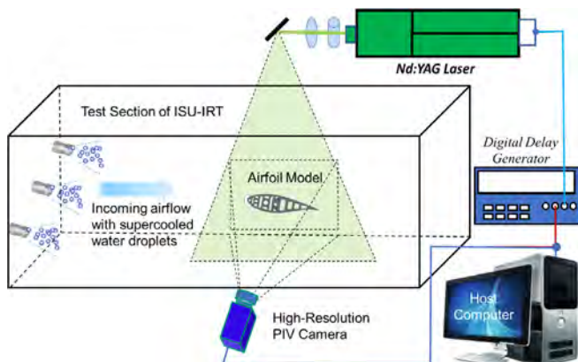
Fig. 2. Experimental setup used for the PIV measurements.
