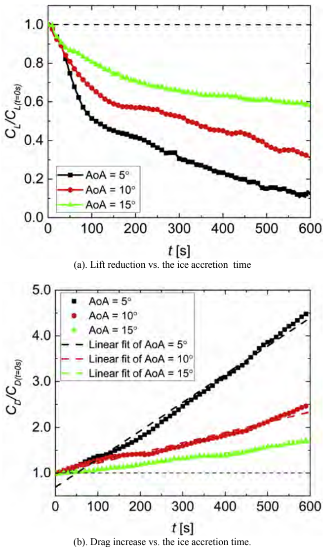
Fig. 9. Aerodynamic performance degradation of the test model induced by the ice accretion at different angles of attack.
