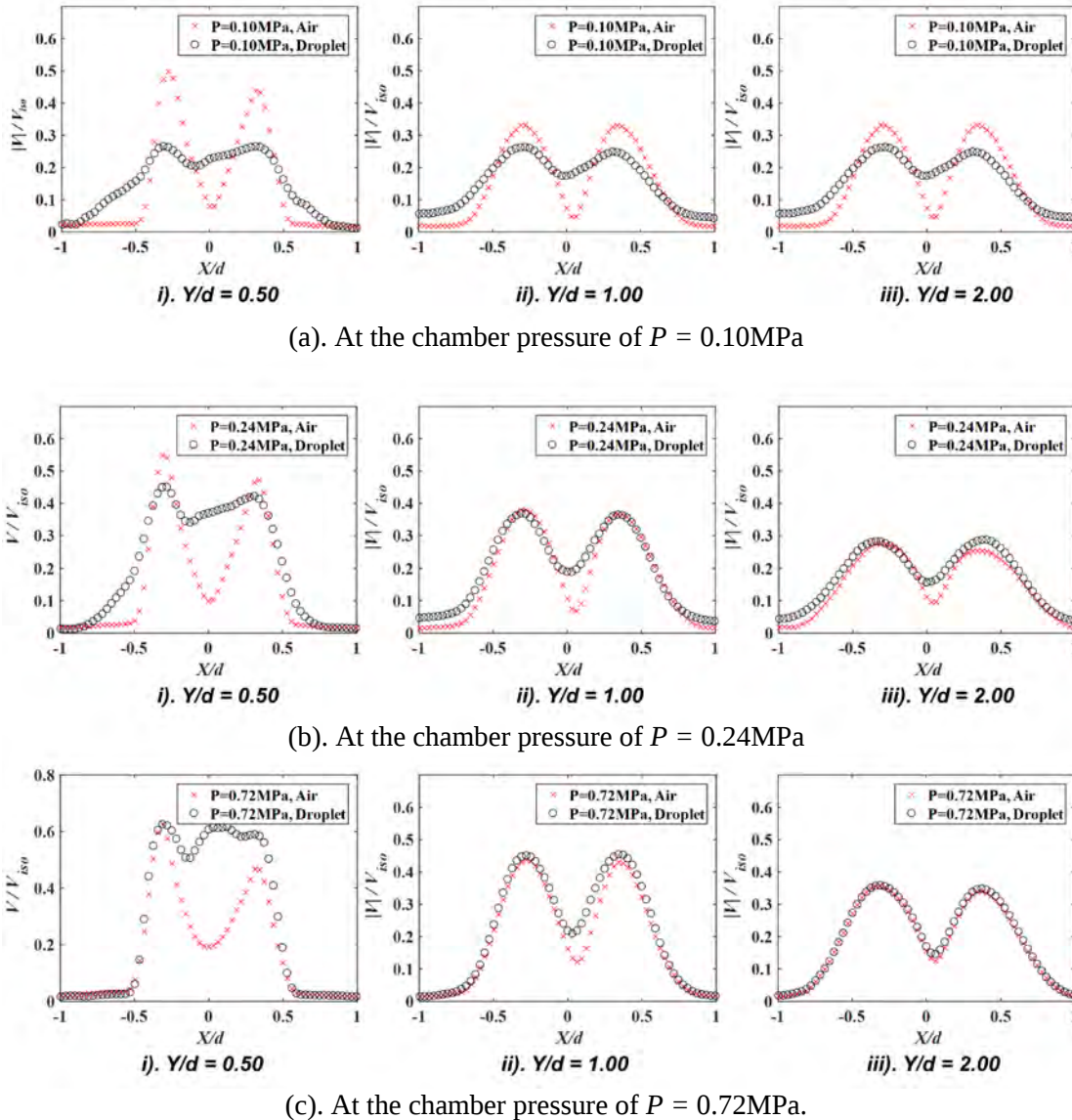
Fig. 5. Transverse velocity profiles of the airflow and spray droplets at three typical downstream locations at different chamber pressures.
