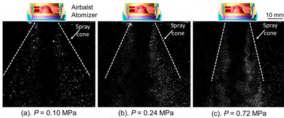
Fig. 8. The acquired images of the spray droplets at different chamber pressures.
