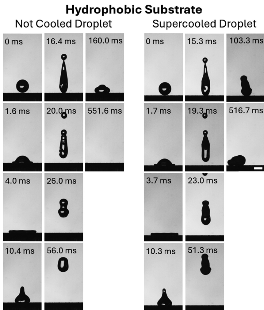
Fig. 10 Time sequence images of droplet impingement on hydrophobic substrates (scale bar: 2 mm). The impact velocity of droplets was measured as V \approx 0.92 m s -1 , We \approx 35 . (left) Droplet was not cooled ( T \approx 4 °C); (right) supercooled droplet ( T \approx -8 °C).
